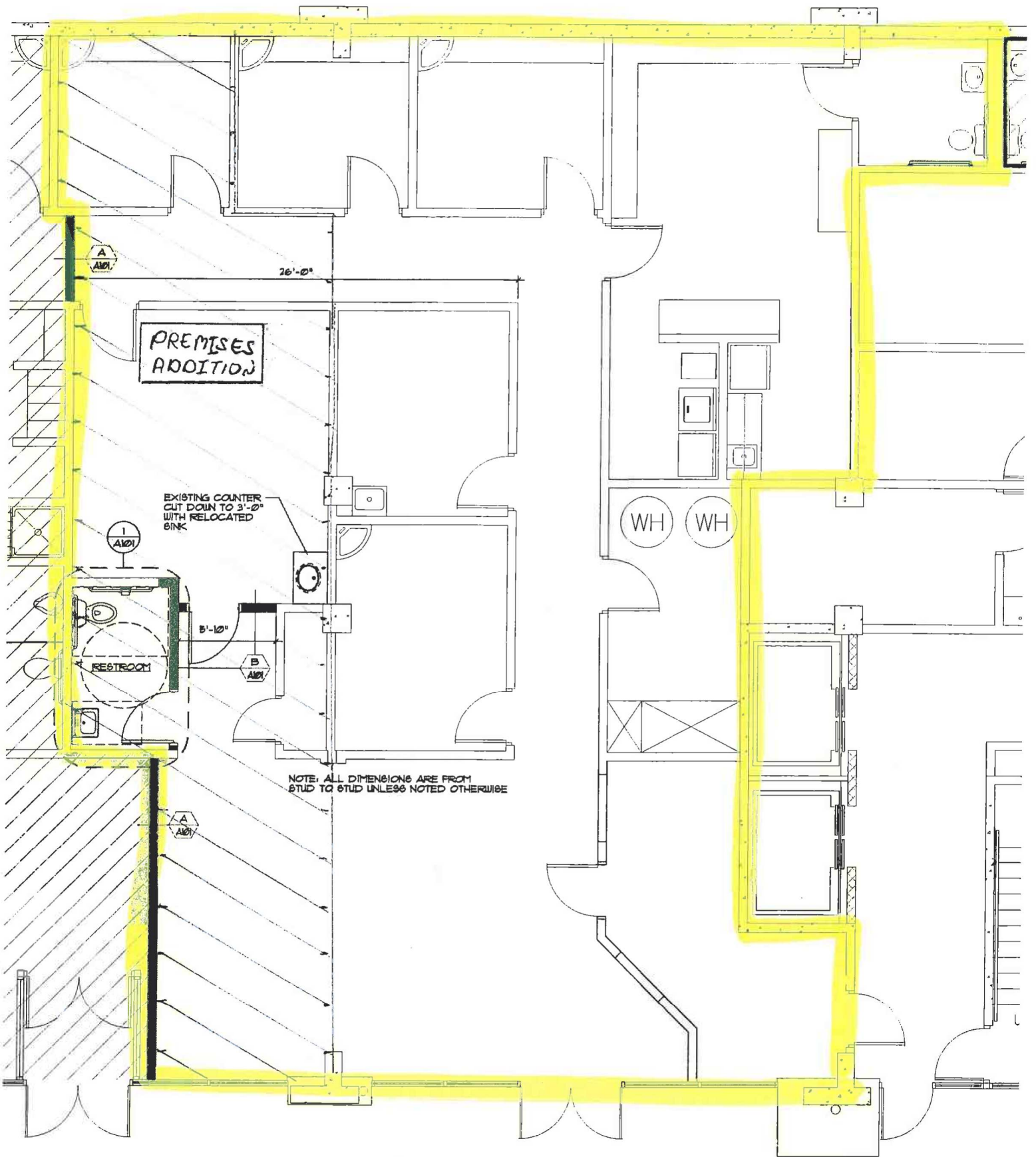
DR. CRITCHLOW RENOVATION FLOOR PLAN SCALE: 1/4" = 1'-0"
